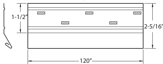
ASS25ML, GSS25ML
